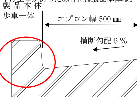
図-2 L型街渠
